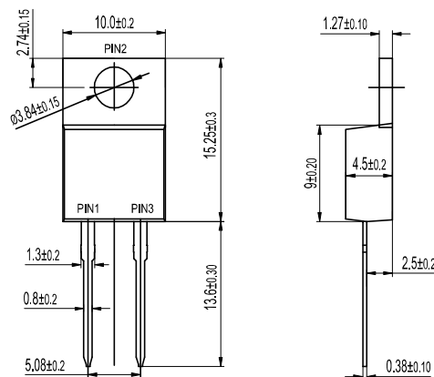
TO-220AC HER8XX
